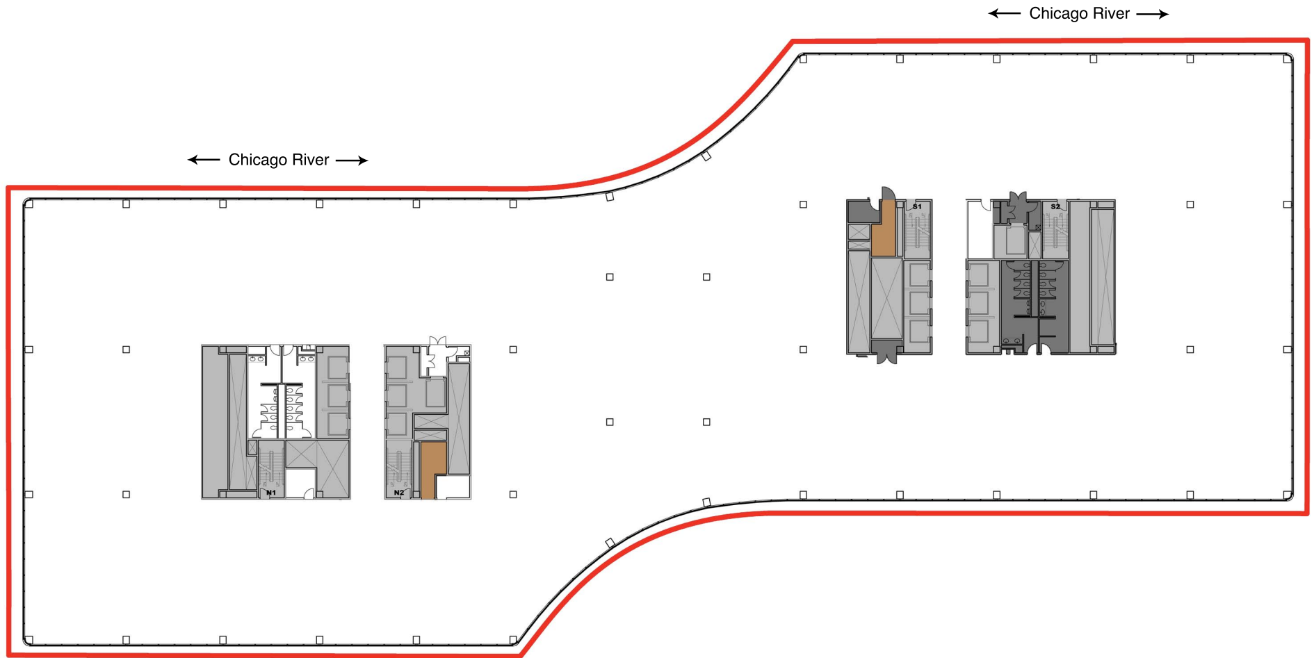
TYPICAL FULL FLOOR PLAN (FLOORS 1-23)
